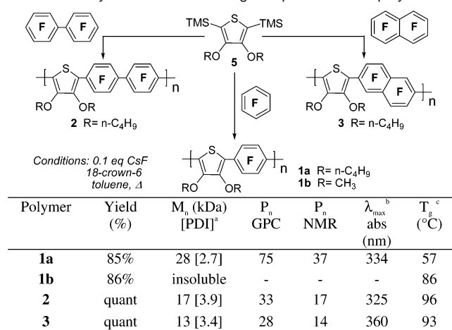
Scheme 1. Synthesis of Alternating Thiophene– \pi F Copolymers.
